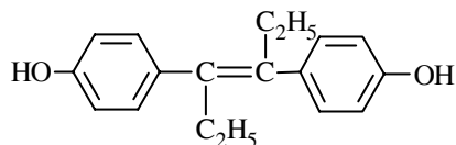
trans- Stilbestrol
