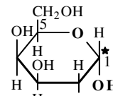
2-Deoxy-D- \alpha - Glucopyranose
