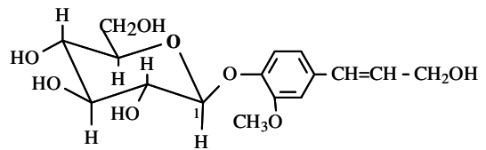
Coniferin- \beta\text{-D-Glucopyranosid}
