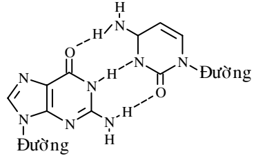
Cặp Guanin-Cytosin
