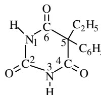
Luminal
