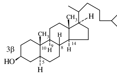
3β-Cholestanol
