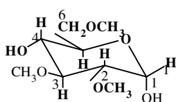
2,3,6-Tri-O-methyl- \alpha -D-Glucose (90%)
