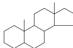
Androstan
