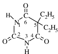
Veronal
