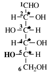
L (-)-Glucose
