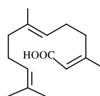
Acid farnesenic
