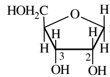
2-Deoxy-D (-)-Ribofuranose
