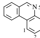
Phenanthridin
