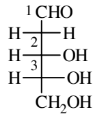
2-Deoxy-D (-)-Ribose
