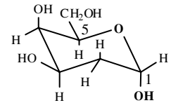
2-Deoxy-D- \alpha - Glucopyranose
