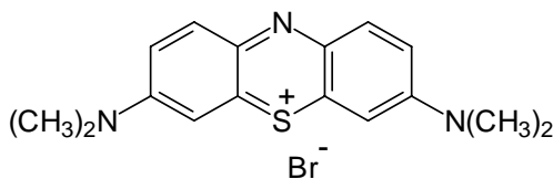
Xanh methylen
