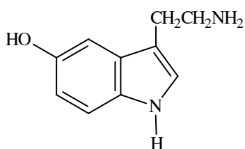
Serotonin
