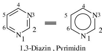
1,3-Diazin, Pyrimidin
